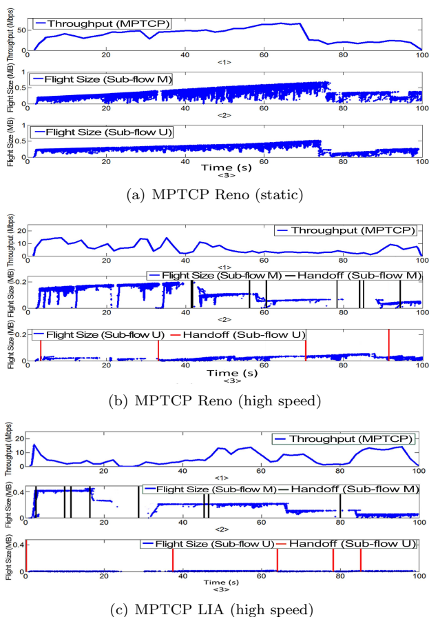
Figure 12: Variation in throughput and flight size of MPTCP over time
