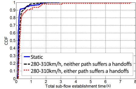
Figure 8: CDF of total sub-flow establishment time
