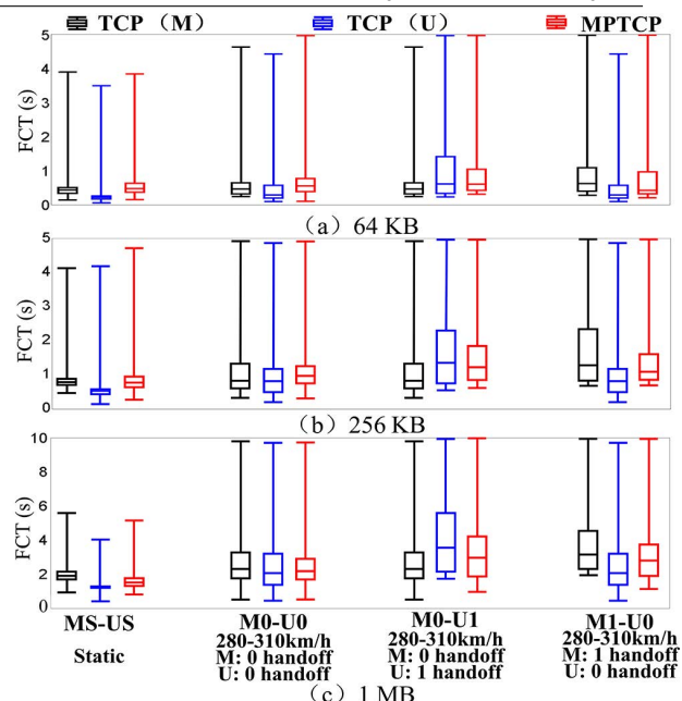
Figure 5: FCT of mice flows
