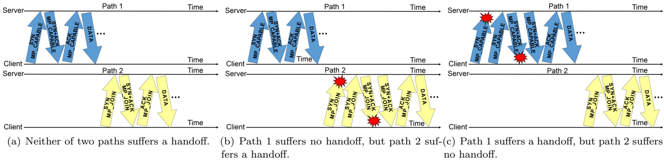
Figure 6: Sub-flow establishment
